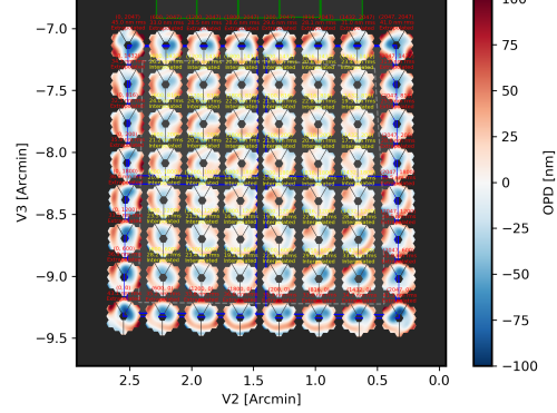
Wavefront model results for NIRCam module A, short wave at 2.0 micron (F200W)
