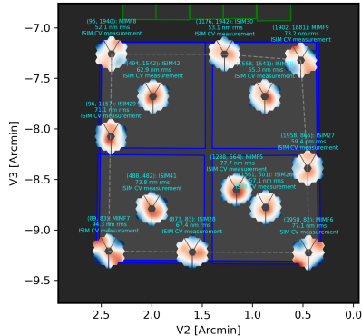
Wavefront model input field points for NIRCam module A, long wave channel at 3.6 micron
