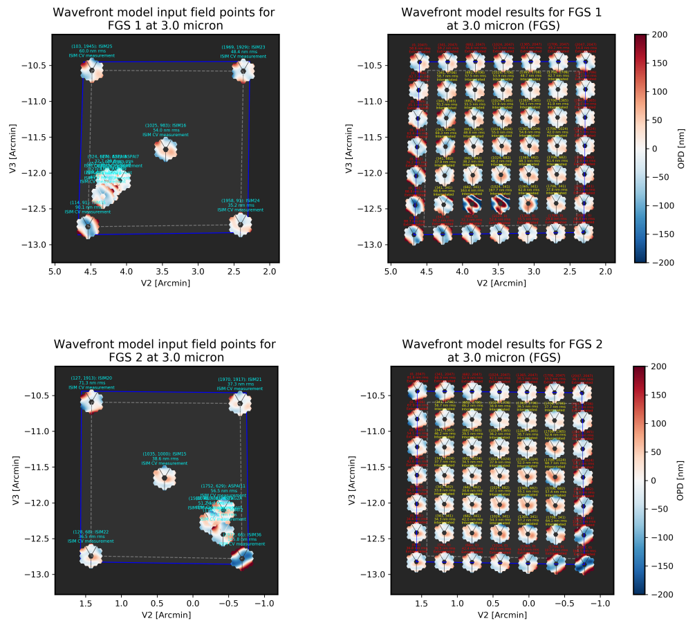
Fig. 6: Instrument WFE models for FGS. Click for full size.
