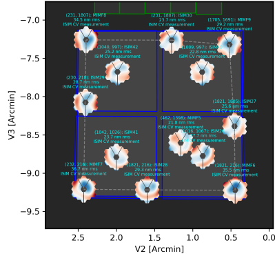
Wavefront model input field points for NIRCam module A, short wave channel at 2.0 micron
