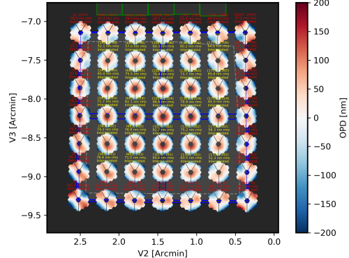
Wavefront model results for NIRCam module A, long wave at 3.6 micron (F356W)
