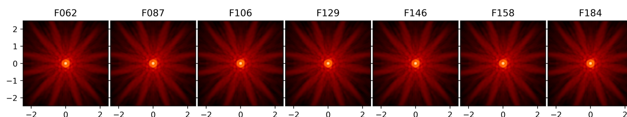
Fig. 1: Sample PSFs for the filters in the WFIRST WFI. Angular scale in arcseconds, log-scaled intensity.
