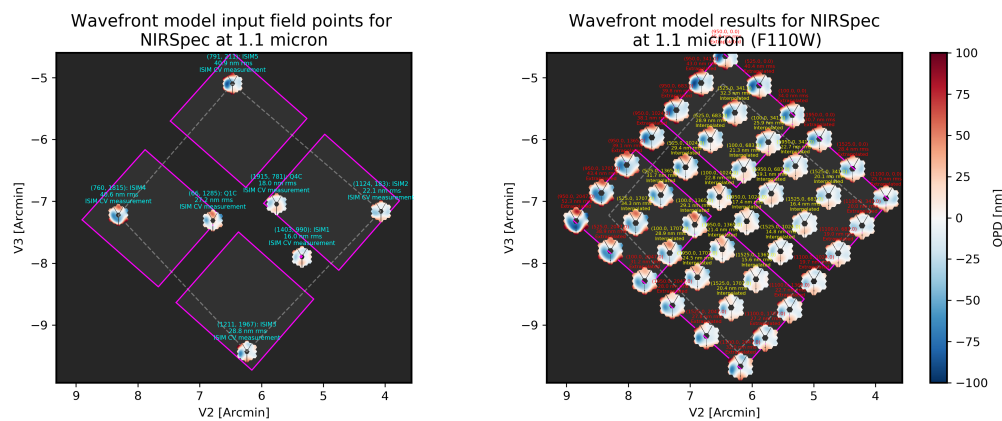
Fig. 3: Instrument WFE models for NIRSpec. Click for full size.
