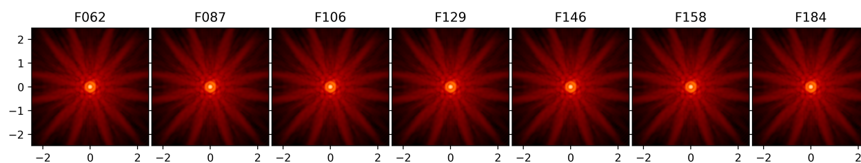
Fig. 2: Sample PSFs for the filters in the WFIRST WFI.
