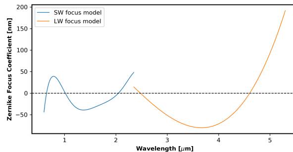
Fig. 2: Instrument focus models for NIRCам. Click for full size.
