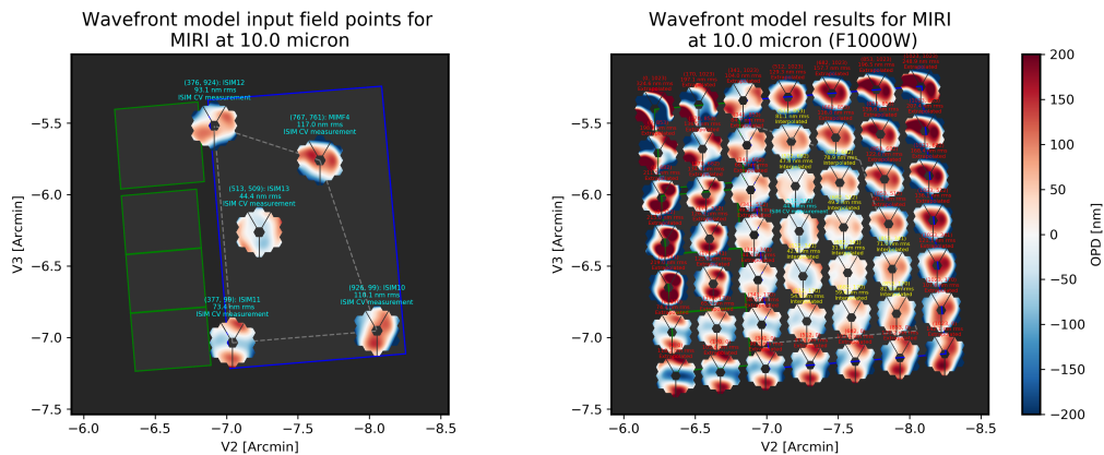
Fig. 5: Instrument WFE models for MIRI. Click for full size.
