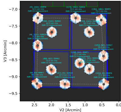
Wavefront model input field points for NIRCcam module A, long wave channel at 3.6 micron
