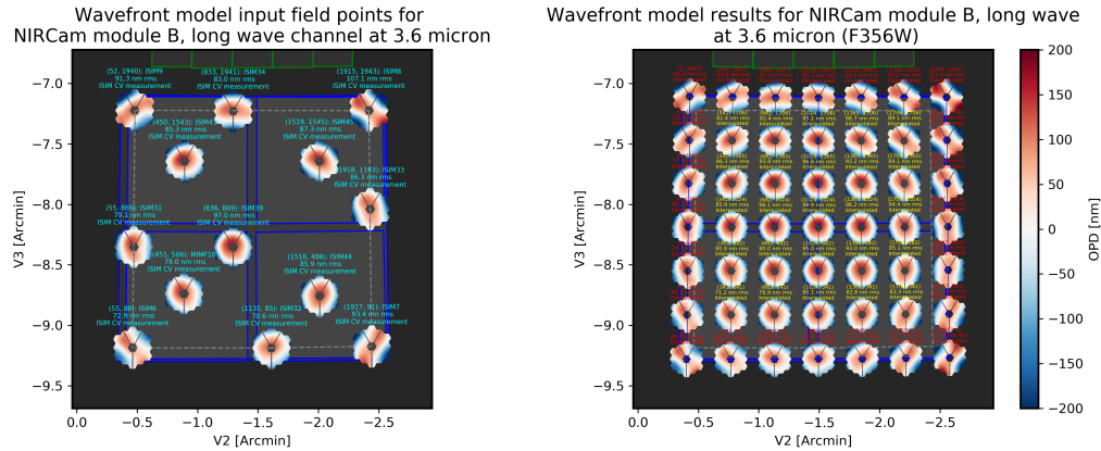
Fig. 1: Instrument WFE models for NIRCам. Click for full size.
